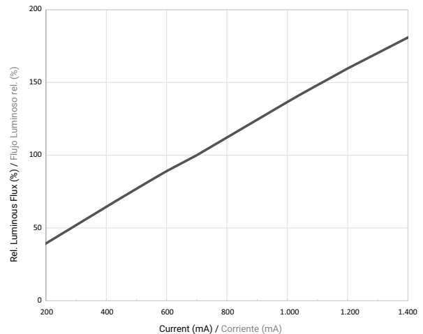
Rel. Luminous Flux vs. Current Flujo Luminoso rel. vs. Corriente
