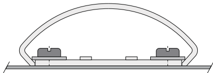
Diffuser fixing with M4 insulation ring Fijación del difusor mediante arandela de plástico M4 ( Ref. 9710107 DIN-125 M4 x \varnothing 4,30 x \varnothing 9 x 0,80 6.6PA )
